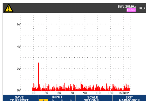
Extended harmonics spectrum from 9 kHz to 150 kHz
