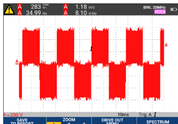
Drive output waveform with auto triggering
