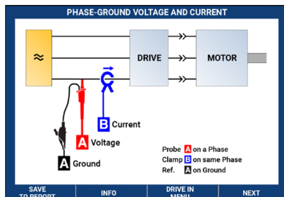
Drive input step-by-step guided measurement connections
